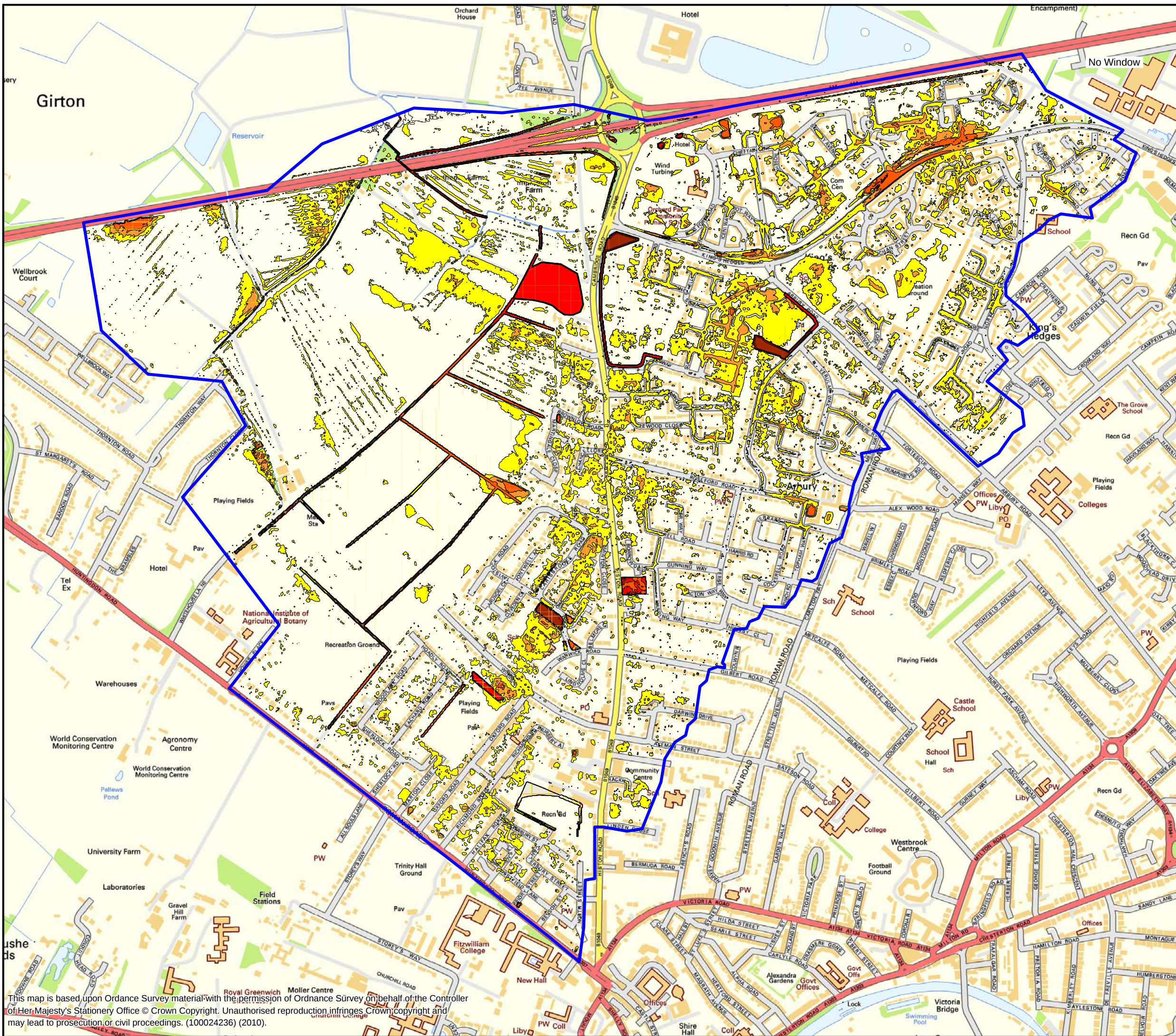
FIGURE F19 0.5% AEP "ENGINEERING OPTION C5" PLUVIAL MODELLING MAXIMUM DEPTH KING'S HEDGES AND ARBURY
